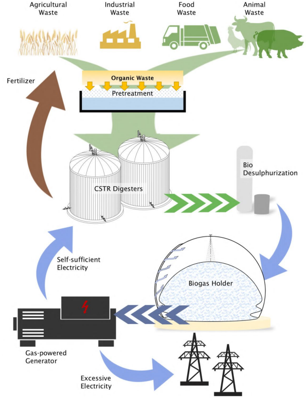
Biogas Diagram: How the Biogas is Produced?
